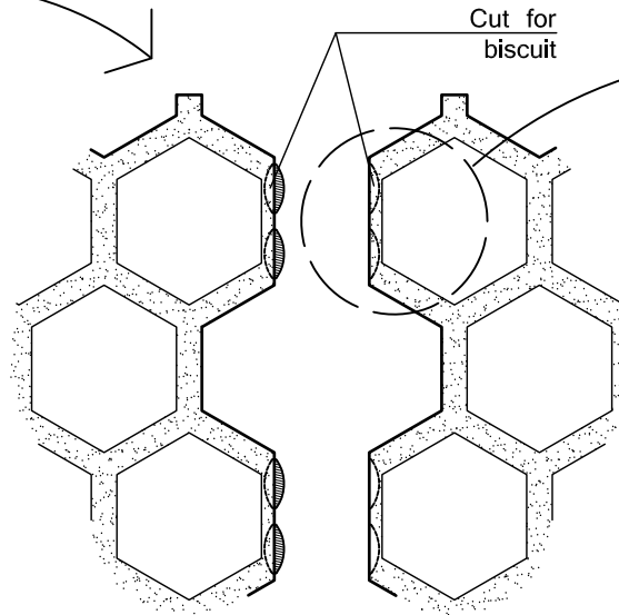
DETAIL JOINT NOT TO SCALE
