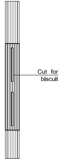
SECTION DETAIL JOINT NOT TO SCALE
