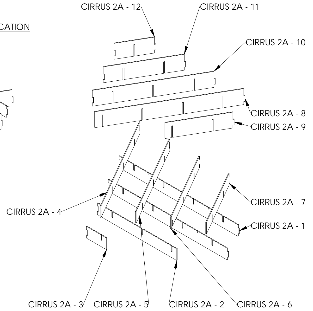
EXPLODED VIEW
