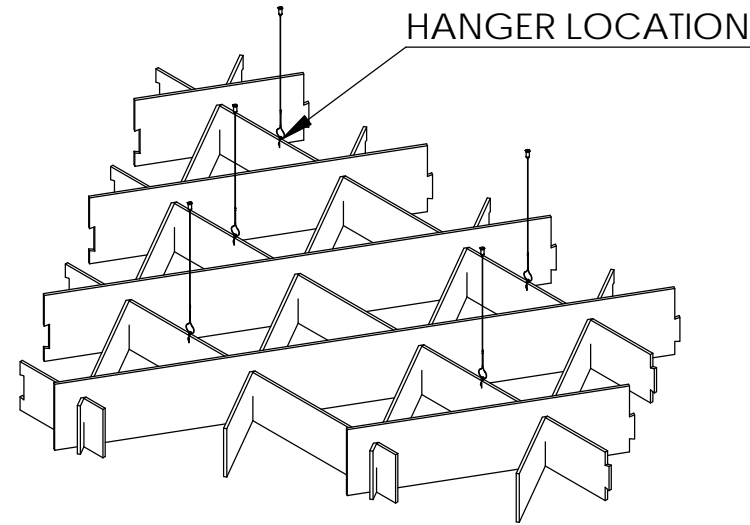
PERSPECTIVE VIEW
